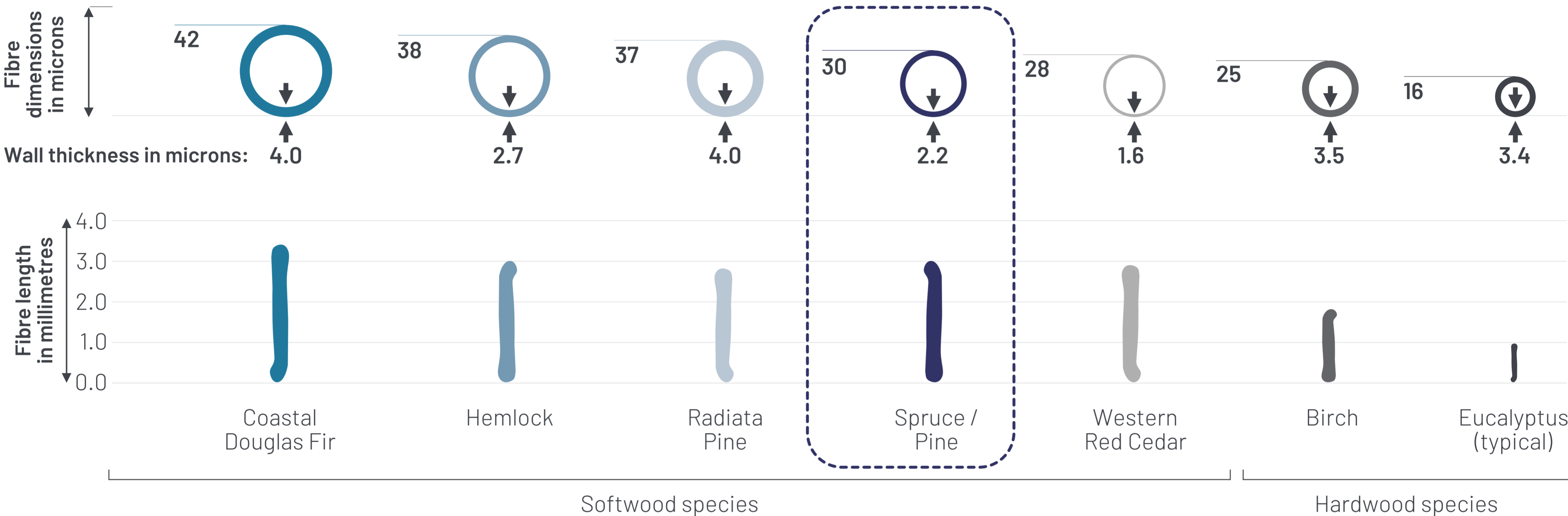
Source: Canfor investor presentation: fibre characteristics, November 2008
